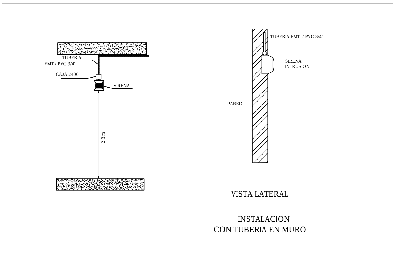
SIRENA ALARMA INTRUSION
